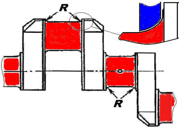
Fig.1. Crankshaft bearings grinding devices' placement
