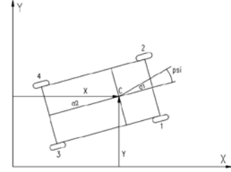
Fig. 3 Plane model describing only the slip angle
