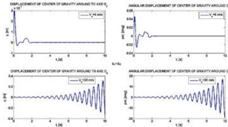
fig. 13 Displacements are around the axes O_y and the Angular displacement around the axes O_z Distance from CG to front axel a_1 = 1.2 , V_{cr} = 0 km / h, with disturbing force
