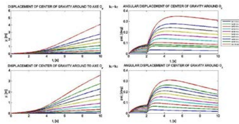
fig. 7 Displacements are around the axes O_y and the Angular displacement around the axes O_z Distance from CG to front axel a_1 = 1.2 , V_{cr} = 0 km / h, with disturbing force
