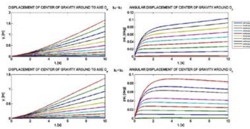
fig. 8 Displacements are around the axes O_y and the Angular displacement around the axes O_z Distance from CG to front axel a_1 = 1.3 , V_{cr} = 294 km / h
