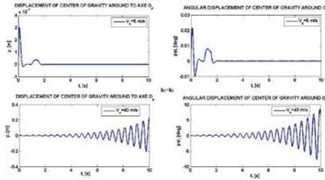
fig. 12 Displacements are around the axes O_y and the Angular displacement around the axes O_z Distance from CG to front axel a_1 = 1.2 , V_{cr} = 0 km / h, with disturbing force
