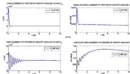
fig. 15 Displacements are around the axes O_y and the Angular displacement around the axes O_z Distance from CG to front axel a_1 = 1.3 , V_{cr} = 294 km / h
