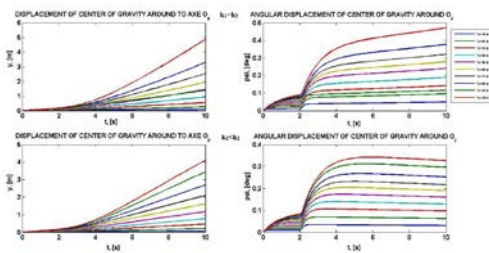
fig. 9 Displacements are around the axes O_y and the Angular displacement around the axes O_z Distance from CG to front axel a_1 = 1.3 , V_{cr} = 294 km / h, with disturbing force
