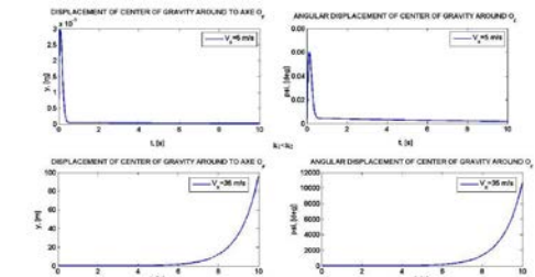
fig. 11 Displacements are around the axes O_y and the Angular displacement around the axes O_z Distance from CG to front axel a_1 = 1.2 , V_{cr} = 0 km / h
