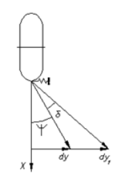
Fig. 5 Plane model about lateral elasticity and slip angle
