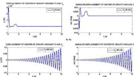
fig. 16 Displacements are around the axes O_y and the Angular displacement around the axes O_z Distance from CG to front axel a_1 = 1.3 , V_{cr} = 294 km / h, with disturbing force
