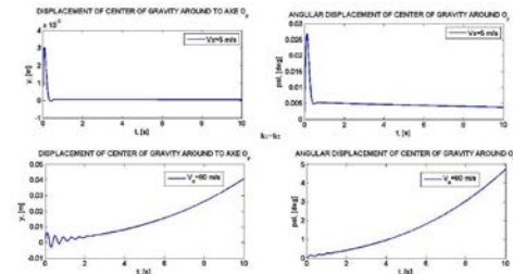
fig. 10 Displacements are around the axes O_y and the Angular displacement around the axes O_z Distance from CG to front axel a_1 = 1.2 , V_{cr} = 0 km / h
