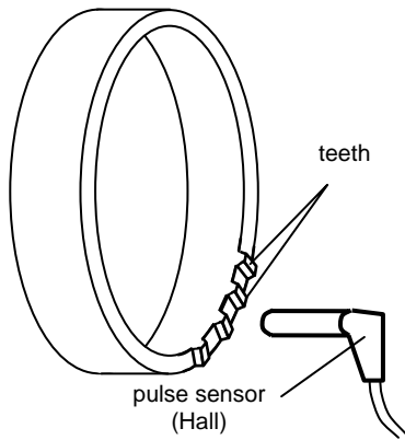
Figure 1 Wheel speed measuring system
