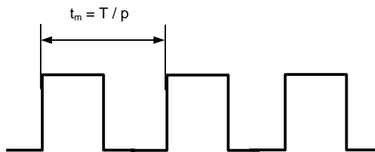
Figure 2 Waveform of signal delivered by wheel speed measuring system
